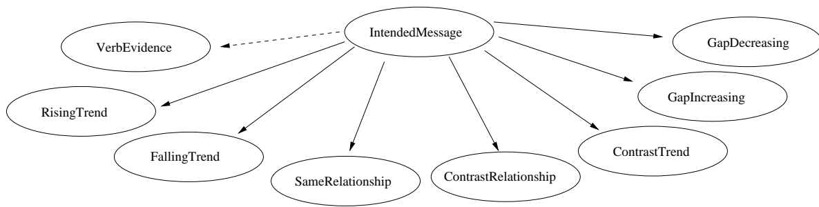
Figure 9: Top level of the Bayesian network.
