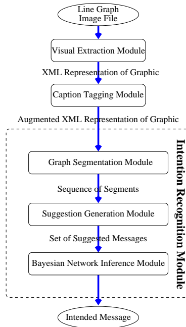
Fig. 3: Overall Architecture
