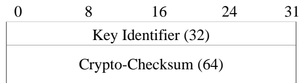
Figure 8. Authenticator Format
