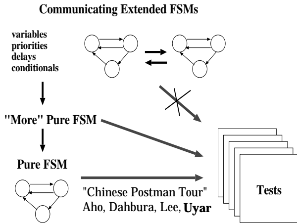
Figure 5: Test generation from Extended FSM
