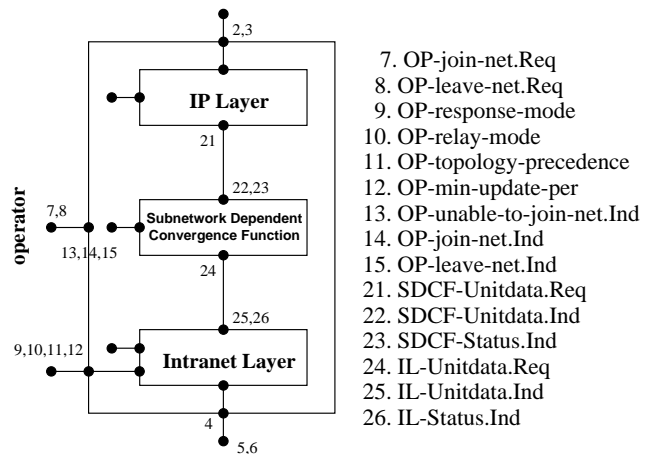
Figure 2: Network Layer Architecture
