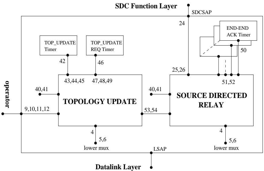
Figure 3: Intranet Layer Architecture
