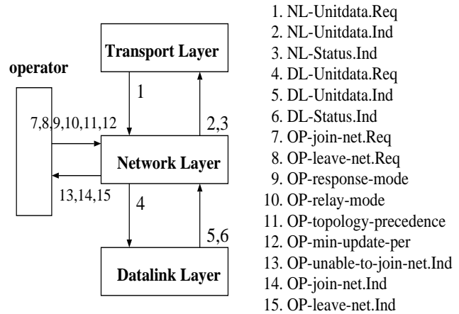
Figure 1: Network Layer Interface
