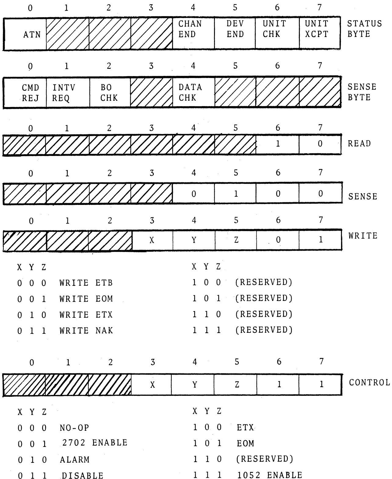
FIGURE 7. DATA CONCENTRATOR CHANNEL COMMANDS.
