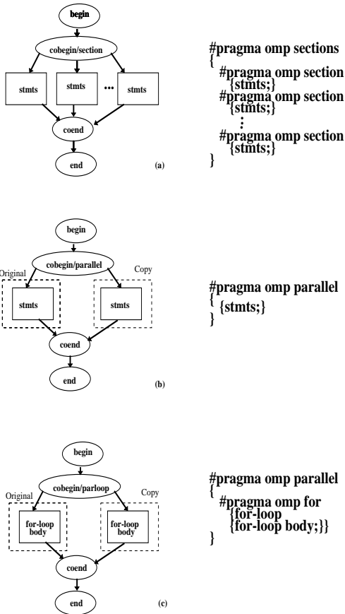
Figure 1. OpenMP (a) Sections (b) Parallel (c) For Modeled as Cobegin/Coend
