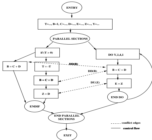
Figure 2. Example CCFG with Conflict Edges
