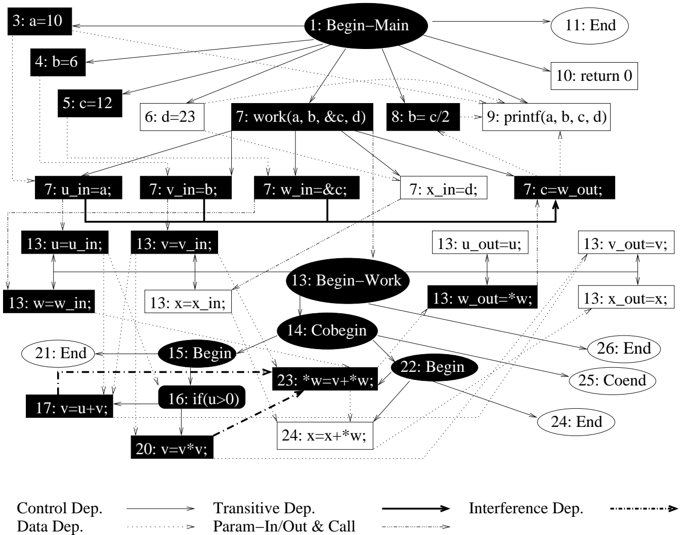
Figure 6. tSDG Program Slice of Example Multi-Procedure OpenMP Program
